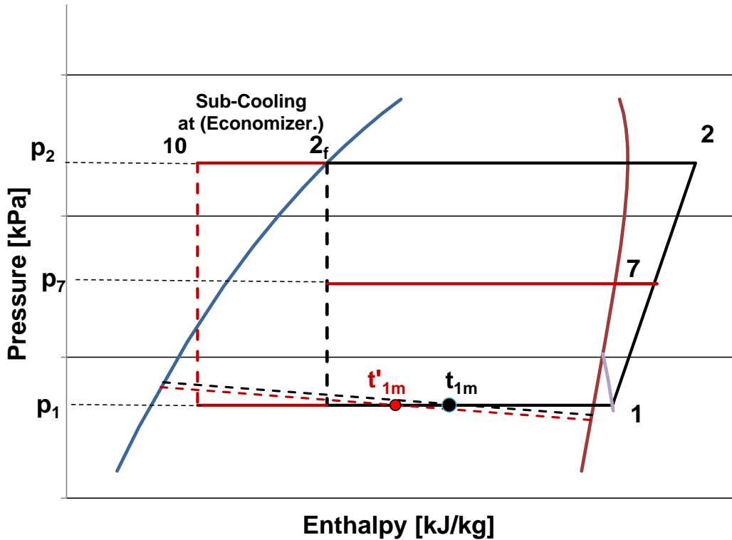
Figure 4: Effect of the Economizer outlet temperature on Evaporating mid-point temperature
