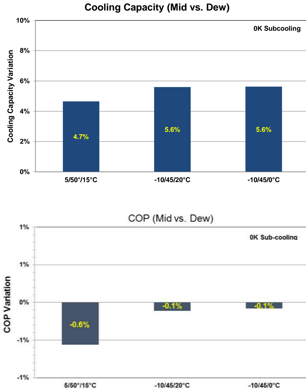
Figure 6: Reciprocating and Scroll Compressor performance variations according to dew and mid temperatures
