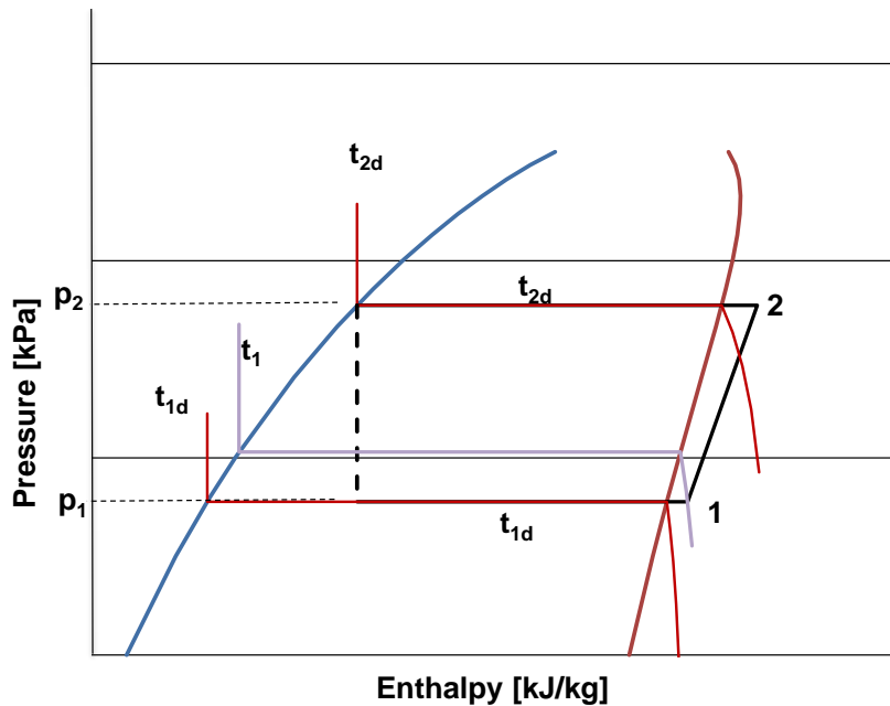
Figure 1: p-h diagram for azeotropic mixture evaporating pressure: p_1 ( t_{1d} ), condensing pressure: p_2 ( t_{2d} )
