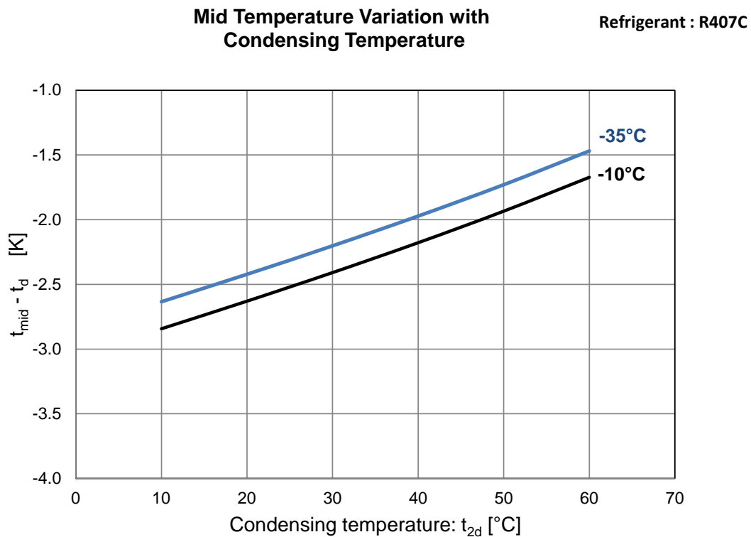
Figure 5: Mid vs. Dew evaporating temperature at various condensing pressure
