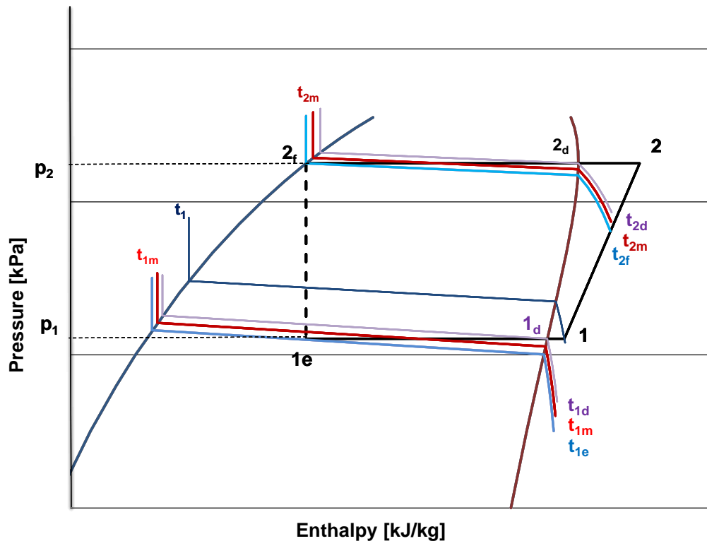
Figure 2: p-h diagram for non-azeotropic mixture
