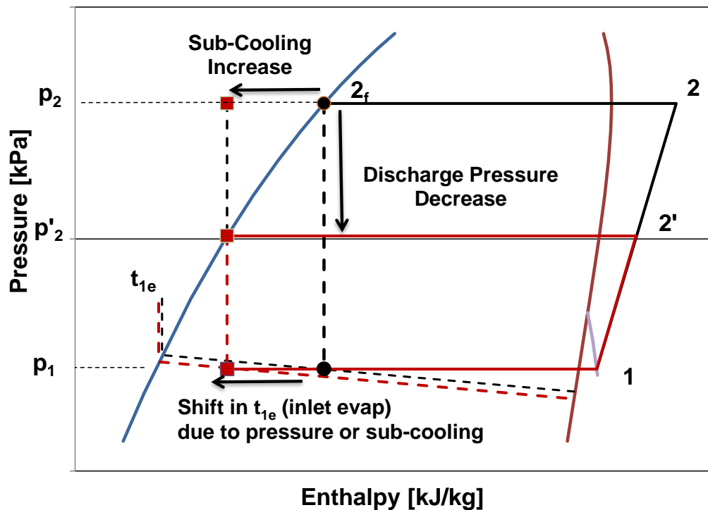
Figure 3: Effect of condensing pressure or the sub-cooling on evaporating mid-temperature
