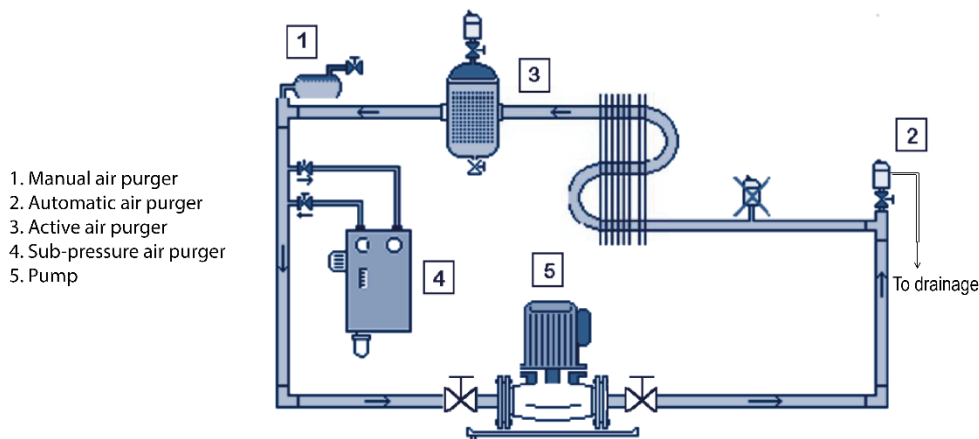
Figure 6. Location of air purgers
